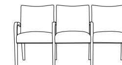
735-33, Three Seat with intervening arm W=66½", D=27", H=33¾", SH=18¼", AH=24¼"
